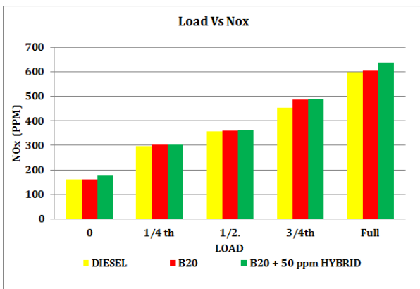
Figure 3. NOx Vs Load
